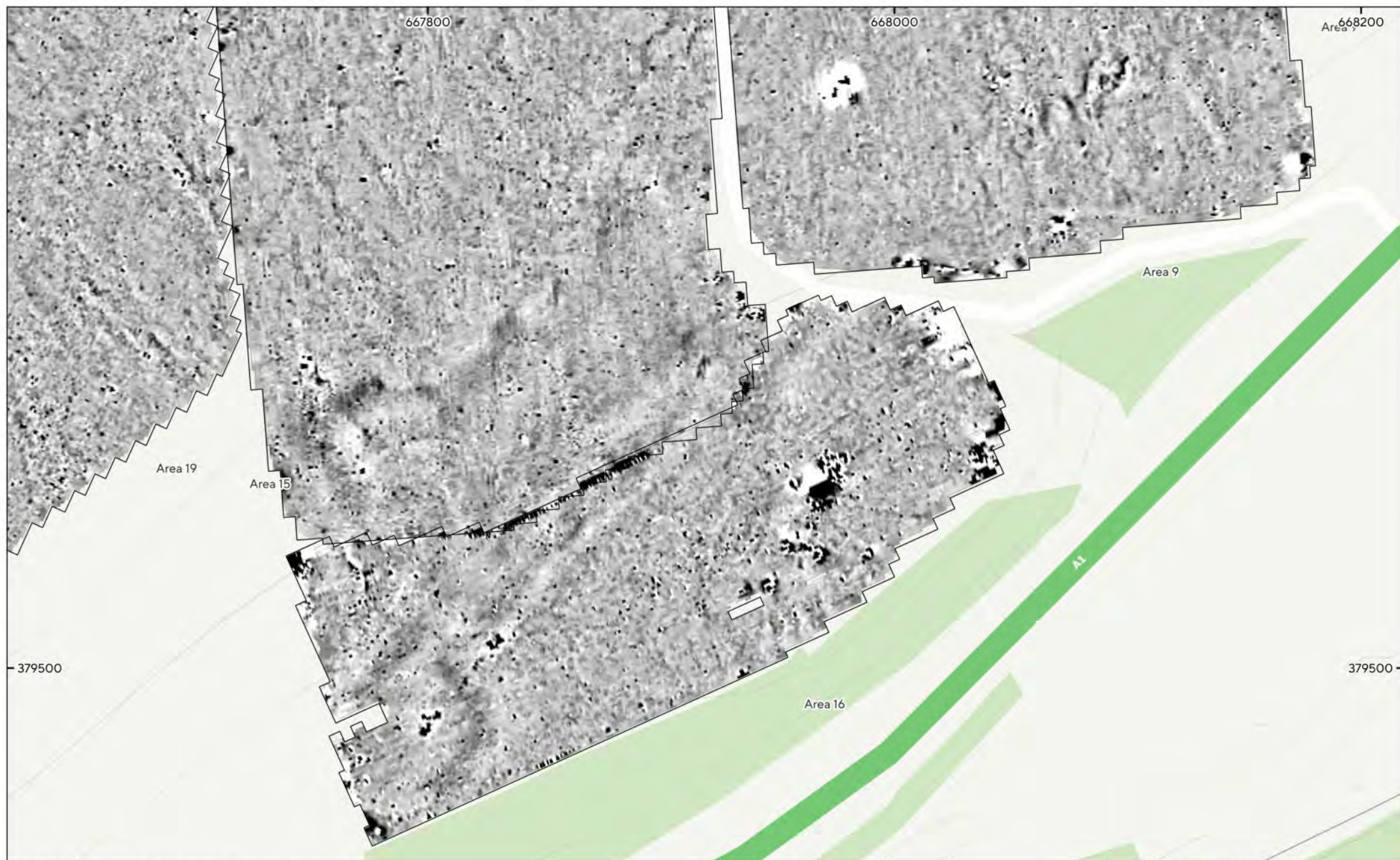
MSNT1874 - Bowshiel, Scottish Borders Figure 35 - Magnetic Gradient (Area 9 & 15 (East), 16, 19 (North-east)) 1:1,500 @ A3 © Magnitude Surveys 2024 Contains Ordnance Survey data © Crown Copyright and database right 2024
