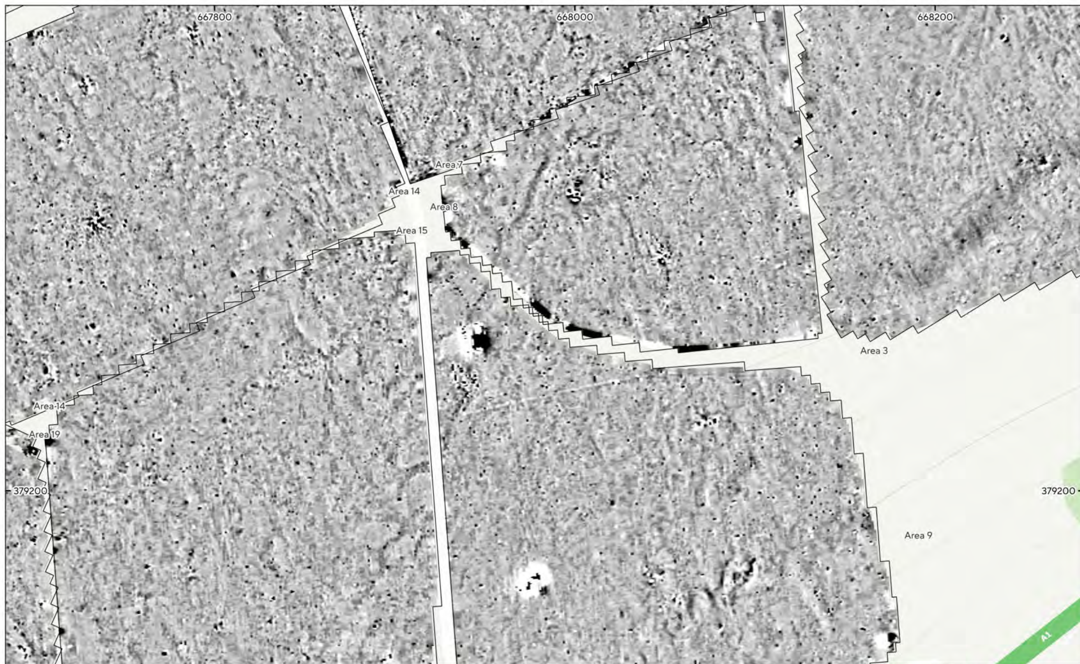
MSNT1874 - Bowshiel, Scottish Borders Figure 39 - Magnetic Gradient (Area 3 (South), 7 (West), 8, 9 & 15 (West), 14 (North-east)) 1:1,500 @ A3 © Magnitude Surveys 2024 Contains Ordnance Survey data © Crown Copyright and database right 2024
