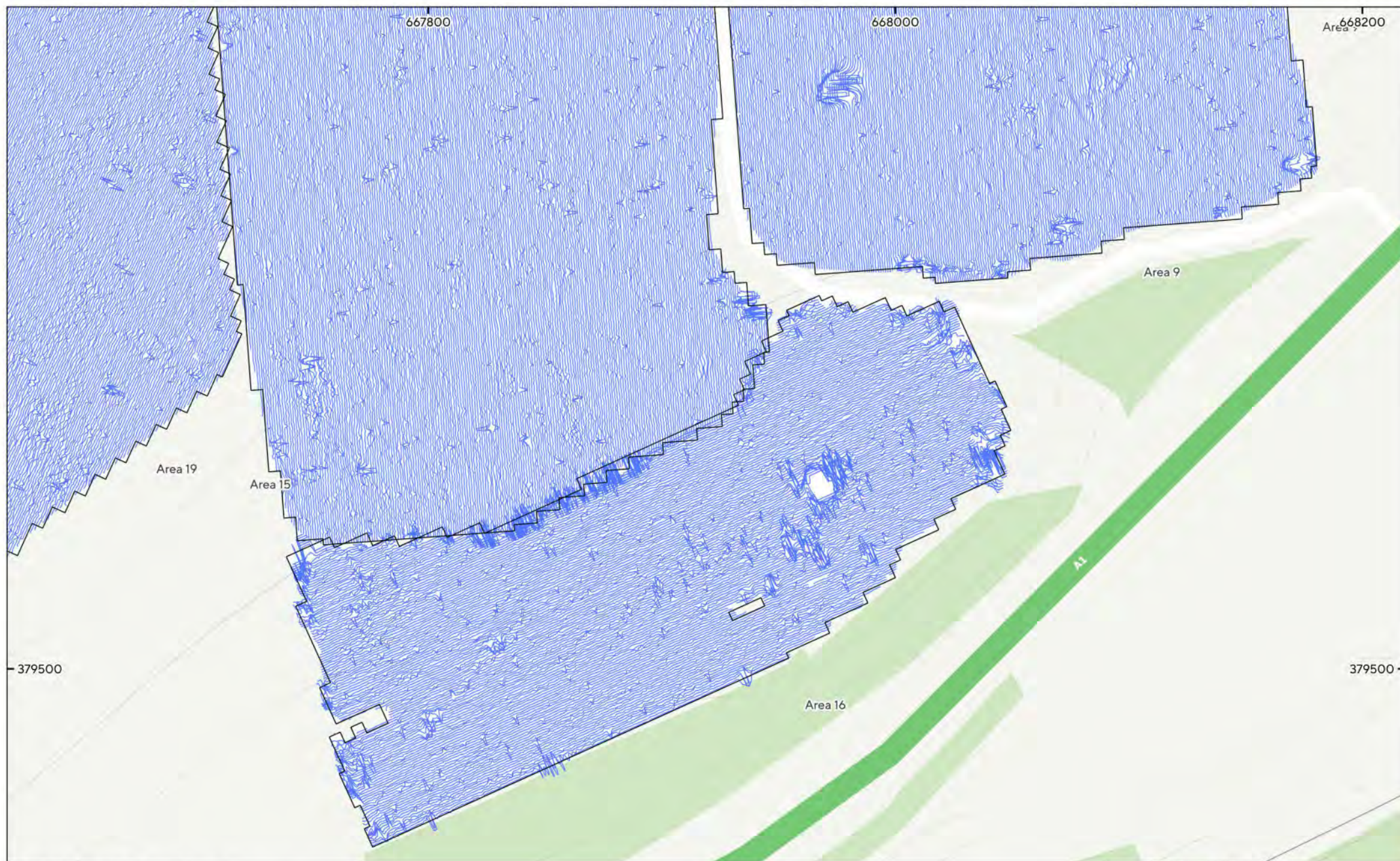
MSNT1874 - Bowshiel, Scottish Borders Figure 37 - XY Plot (Area 9 & 15 (East), 16, 19 (North-east)) 1:1,500 @ A3 30nT/cm at 1:1,500 @ A3 © Magnitude Surveys 2024 Contains Ordnance Survey data © Crown Copyright and database right 2024
