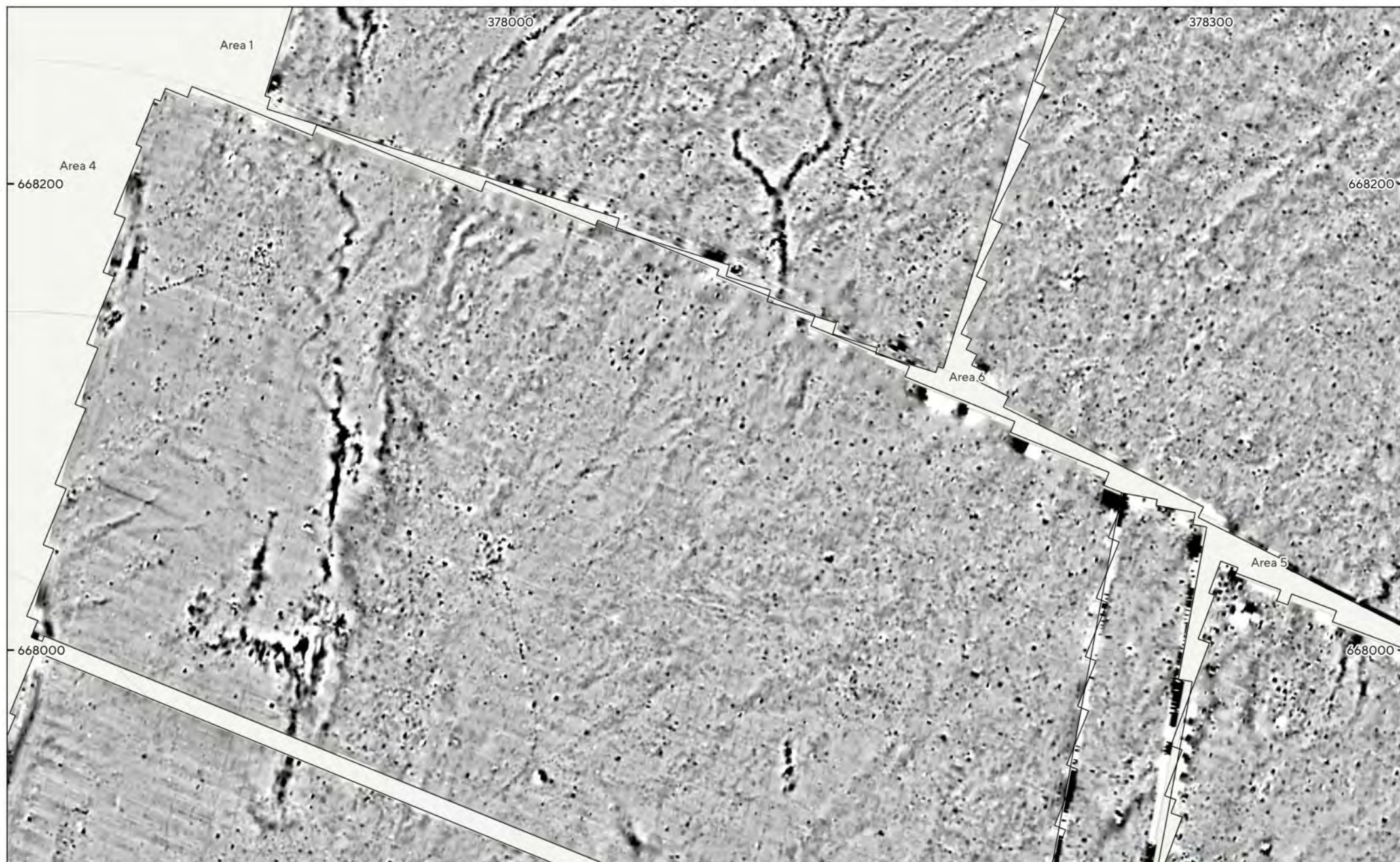
MSNT1874 - Bowshiel, Scottish Borders Figure 31 - Magnetic Gradient (Area 1 (South), 4 (North), 5 & 6 (West), 10 (North)) 1:1,500 @ A3 © Magnitude Surveys 2024 Contains Ordnance Survey data © Crown Copyright and database right 2024
